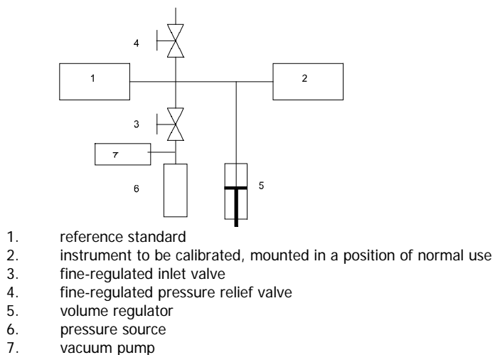
Figure 2 - Set-up in absolute pressure, gaseous media
